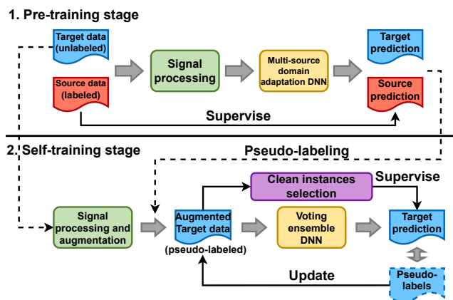
Fig. 2: Framework overview.
